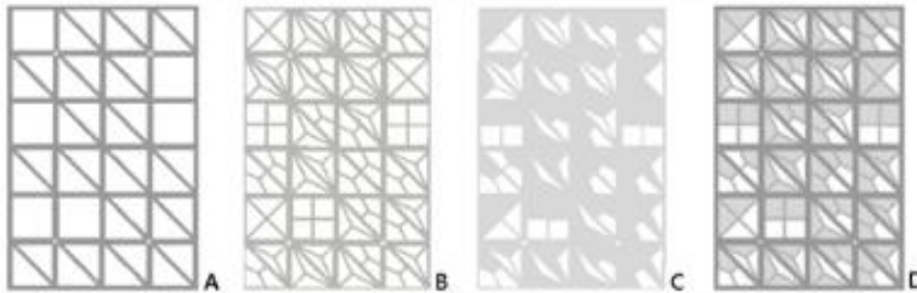
FIG. 10 The set of layers of a panel: A, the outer frame delineating the general shape of the cobogó elements; B, the middle frame outlining their interior elements; C, the inner layer delineating the existing void and opaque areas; D, the wood panel after overlapping the different layers in the following order: A-B-C-B-A.
