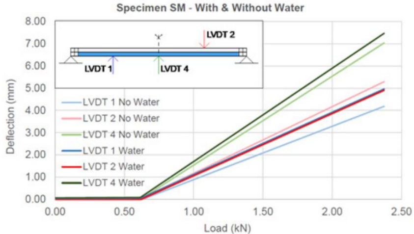
FIG. 16 Deflection of WFG (16 mm water layer) with and without water
